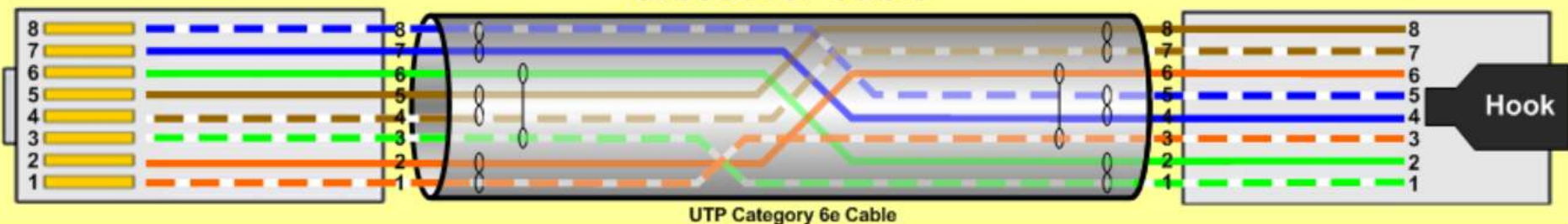
Crossover Cable
