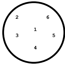
APOLLO RELAY CONNECTOR MCBH-6F-T1 FEMALE FACE VIEW
