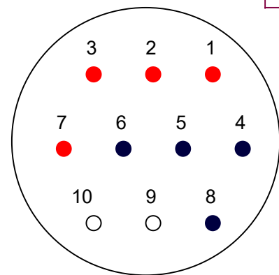
SEACONN-MINM-CCP FEMALE FACE VIEW
