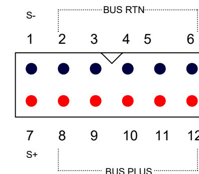
POSITRONIC PLB12M0000 MALE FACE VIEW MALE CRIMP PINS MC116N
