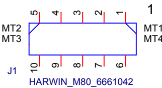
10 Positions Header Connector 0.079" (2.00mm) Surface Mount, Right Angle Gold
