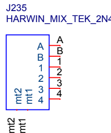
4 Positions Jack 2 Pwr 4 Sig Connector 0.079" (2.00mm) Through Hole Vertical Gold
