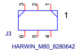
6 Positions Header Connector 0.079" (2.00mm) Surface Mount Vertical Gold
