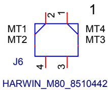
4 Positions Jack Connector 0.079" (2.00mm) Through Hole, Right Angle Gold
