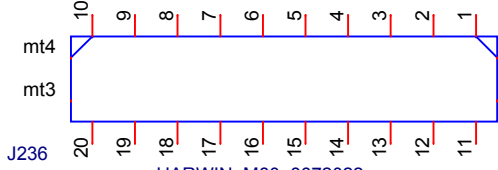
20 Positions Jack Connector 0.079" (2.00mm) Through Hole Vertical Gold With Staples
