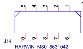
10 Positions Jack Connector 0.079" (2.00mm) Through Hole Vertical Gold
