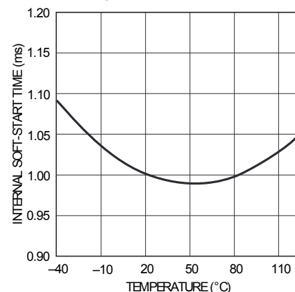
Internal Soft-Start Time vs Temperature
