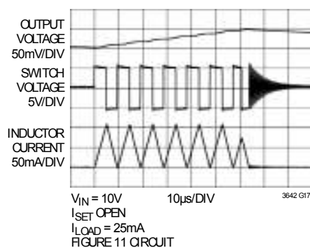
Operating Waveforms
