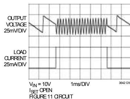
Load Step Transient Response
