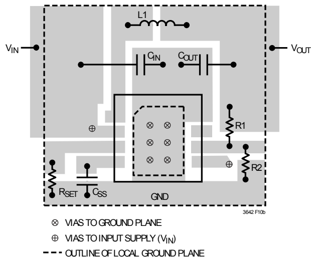
Figure 10. Layout Example
