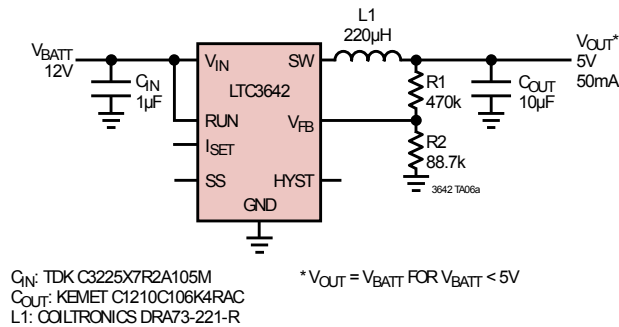
5V, 50mA Regulator for Automotive Applications
