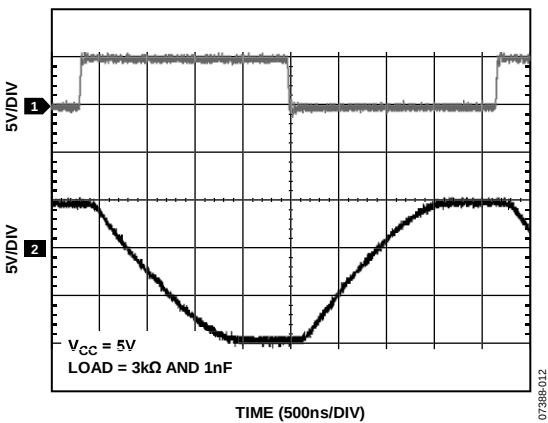
Figure 11. 460 kbps Data Transmission
