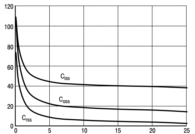
Figure 12. Capacitance
