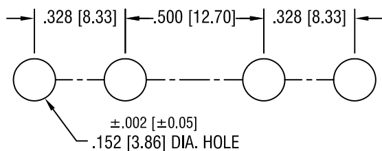
MOUNTING DETAIL
