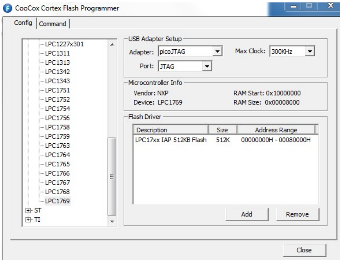
Figure 2.9: Flash Programmer
