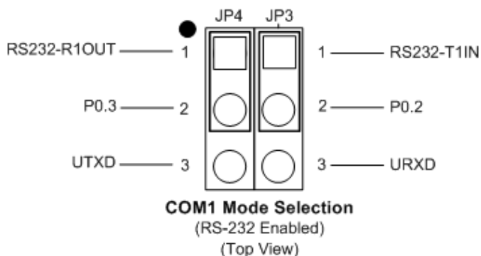
Figure 4.4: COM1 Driver Selection Jumpers
