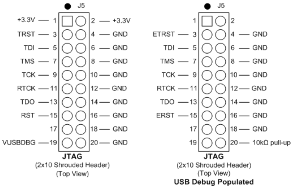
Figure 4.10: JTAG connector pin out
