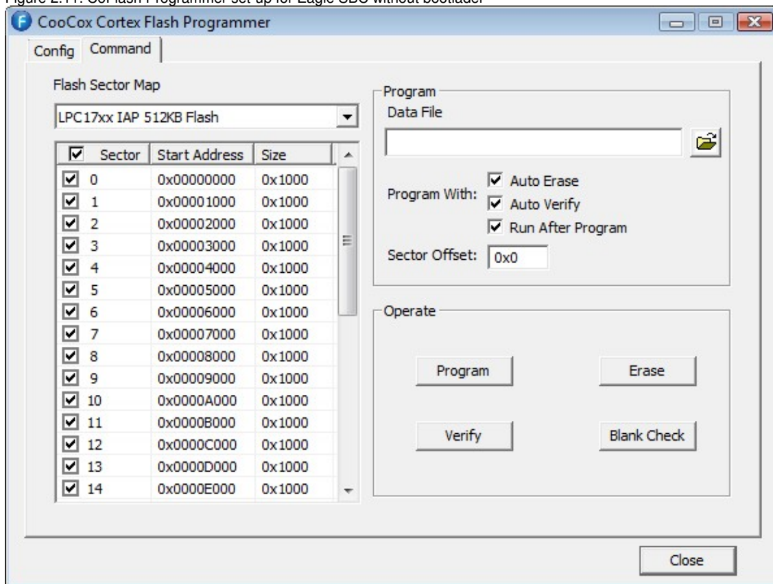
Figure 2.2: CoFlash Programmer set-up for Lincoln SBC
