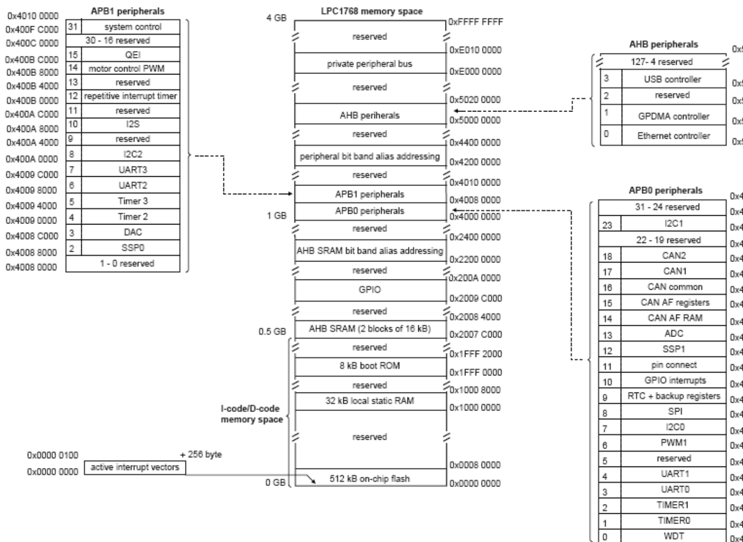
Lincoln 60 Memory Map
