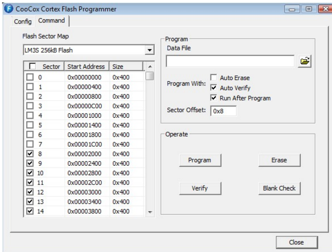
Figure 2.10: CoFlash Programmer set-up for Eagle SBC with bootloader
