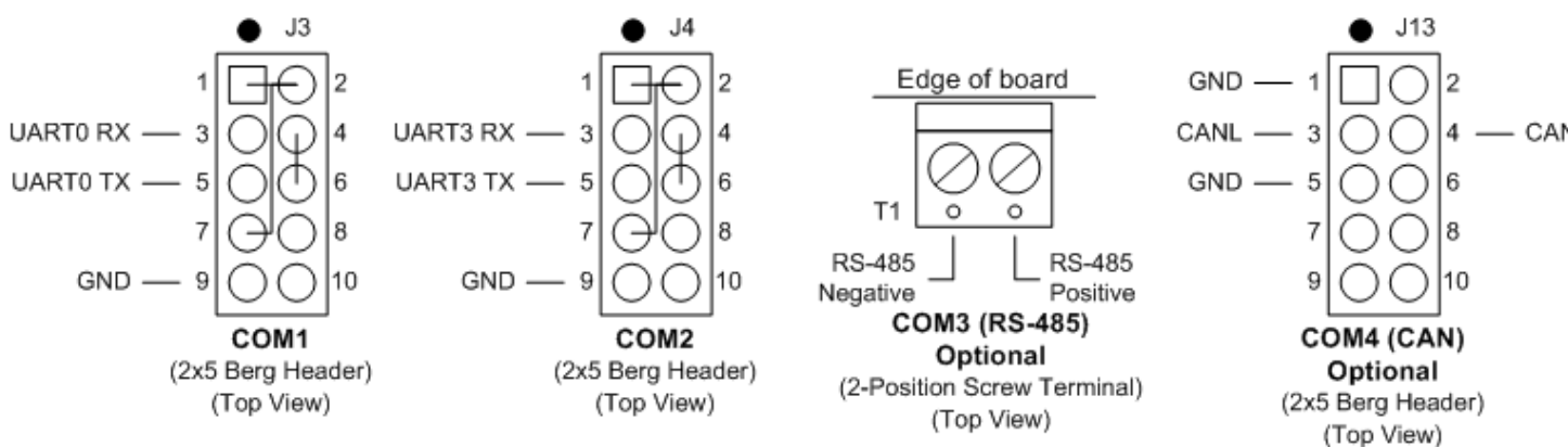
Figure 4.3: COM Ports Connector Pin Outs
