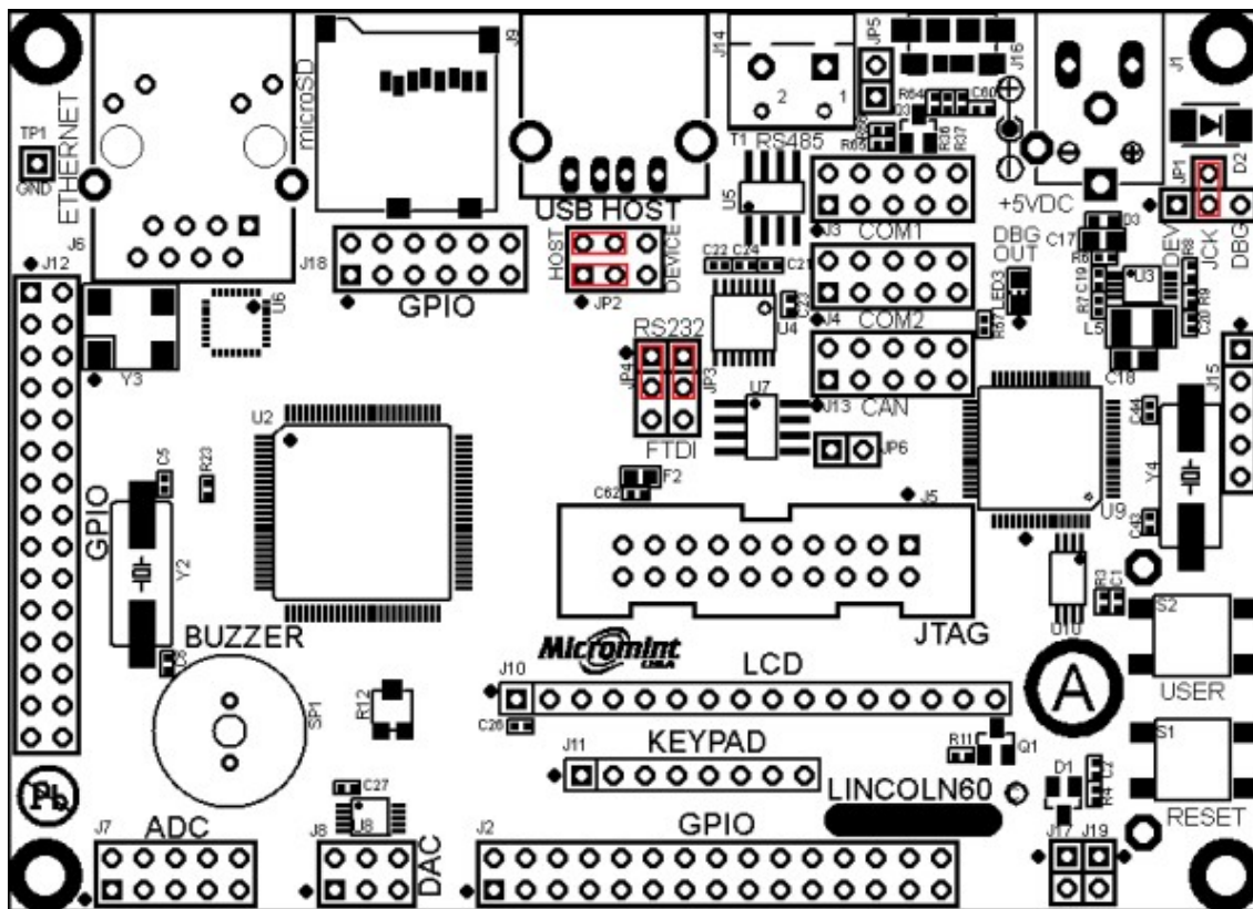
Figure 4.12: Lincoln 60 Base Configuration Default Jumper Settings
