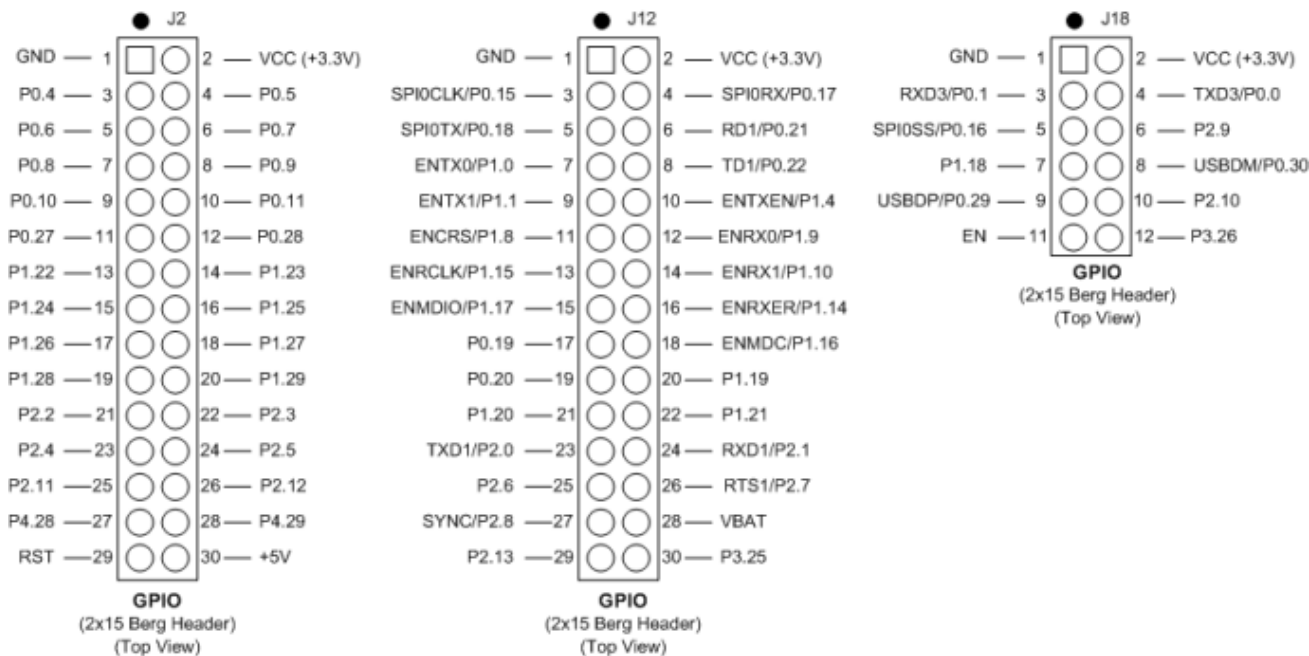
Figure 4.5: GPIO Connector Pin Outs
