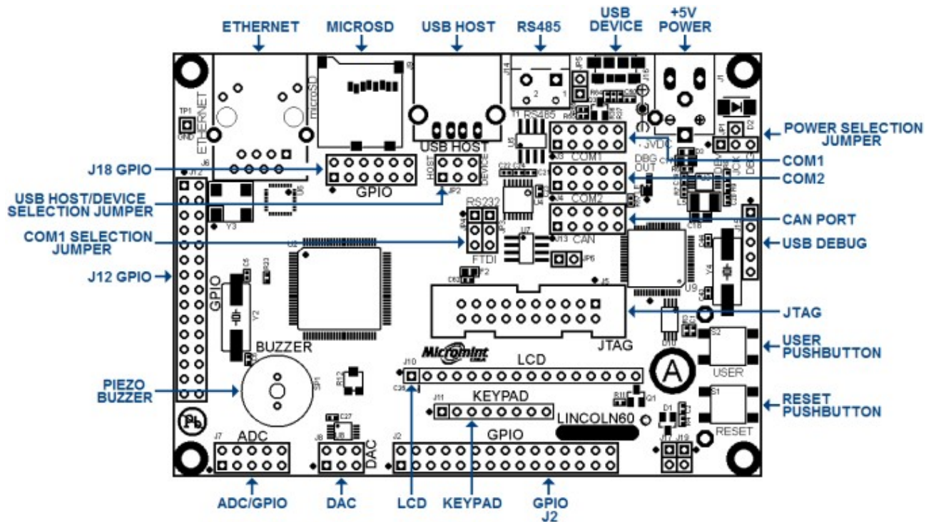
Lincoln 60 User Interfaces, Connectors, and Jumpers
