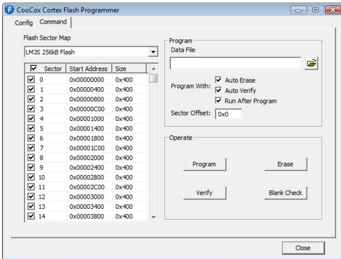
Figure 2.11: CoFlash Programmer set-up for Eagle SBC without bootlader
