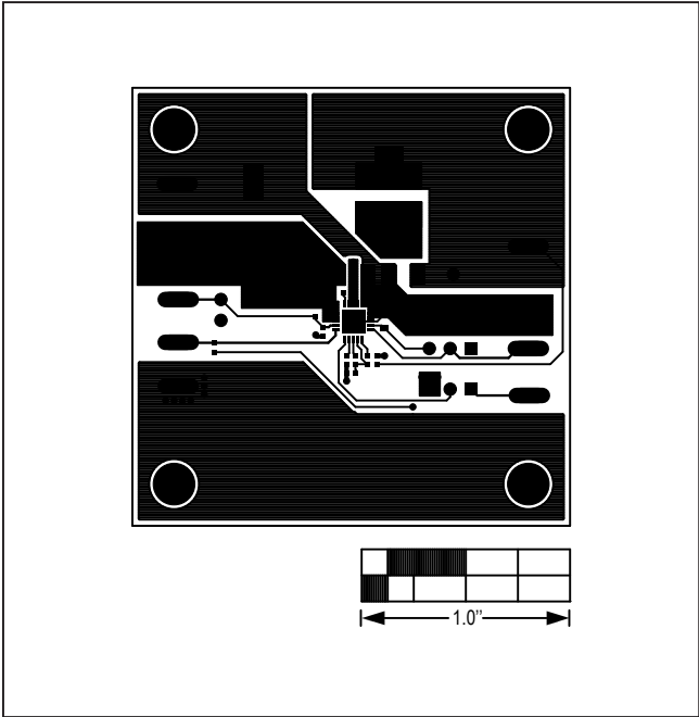
Figure 13. MAX17503 3.3V Output EV Kit Component Side PCB layout
