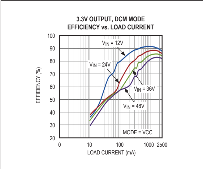
Figure 5. MAX17503 3.3V Output Efficiency (DCM Mode)
