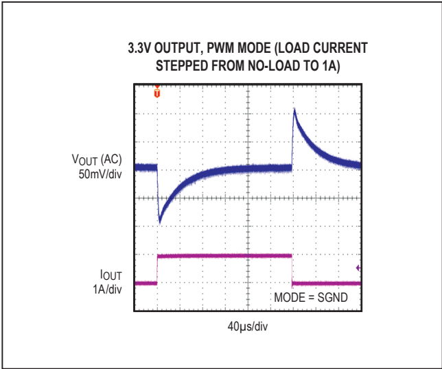
Figure 7. MAX17503 3.3V Output, No Load to 1A Load Transient (PWM Mode)
