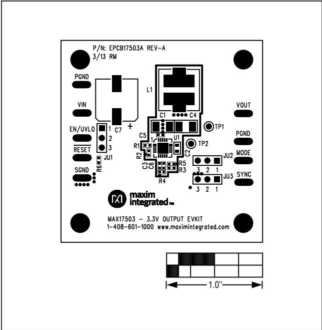
Figure 12. MAX17503 3.3V Output EV Kit Component Placement Guide—Component Side
