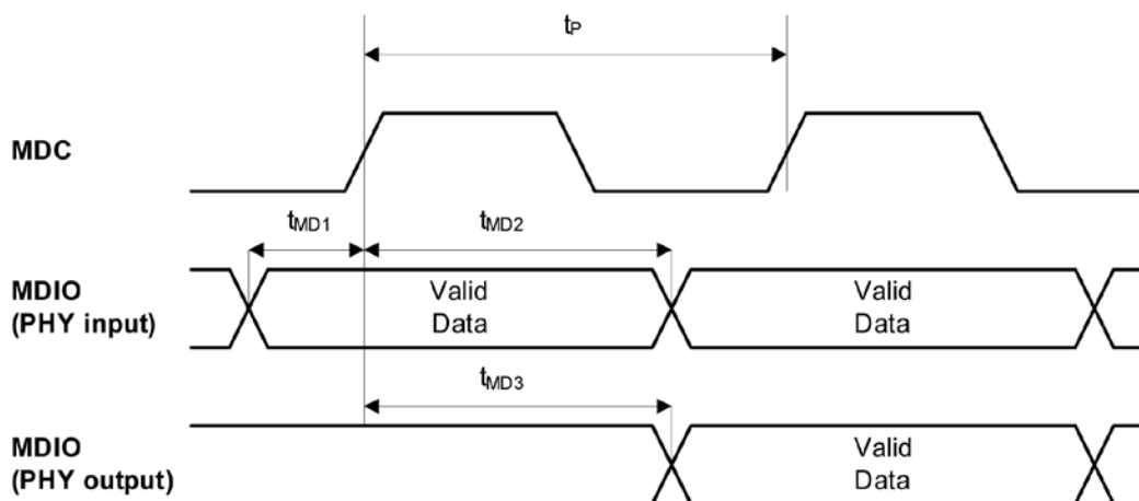
Figure 17. MDC/MDIO Timing
