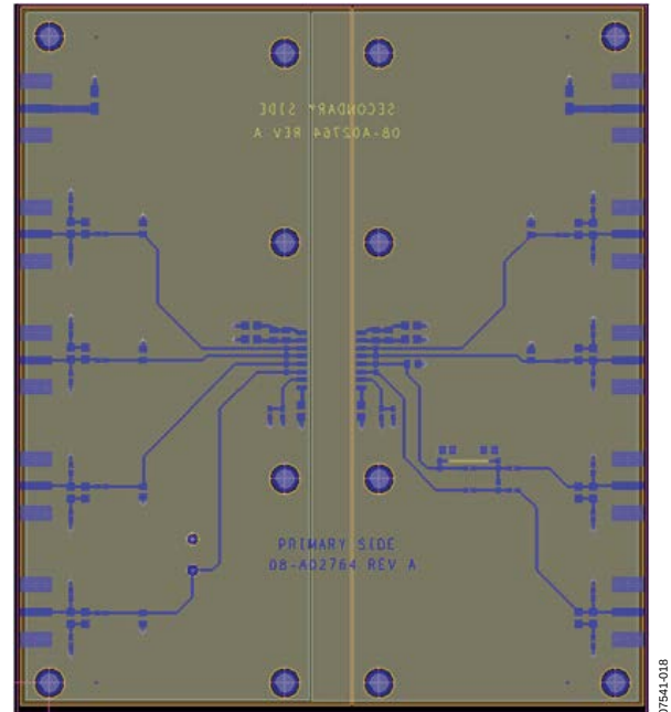
Figure 18. Overlap Stitching Capacitance
