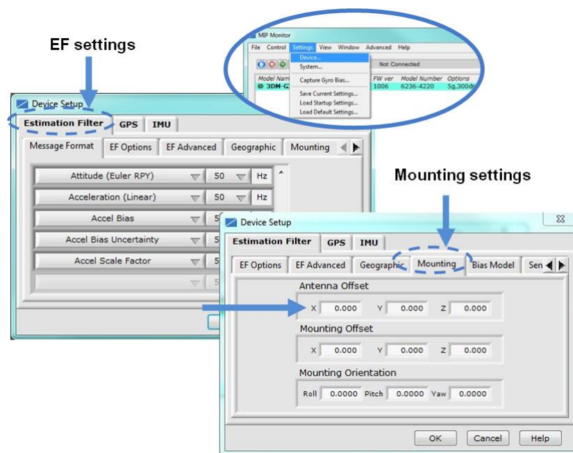
Figure 29 - GPS Antenna Offset
