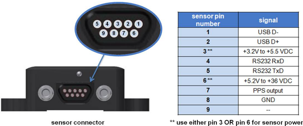
Figure 36 - Connector Wiring
