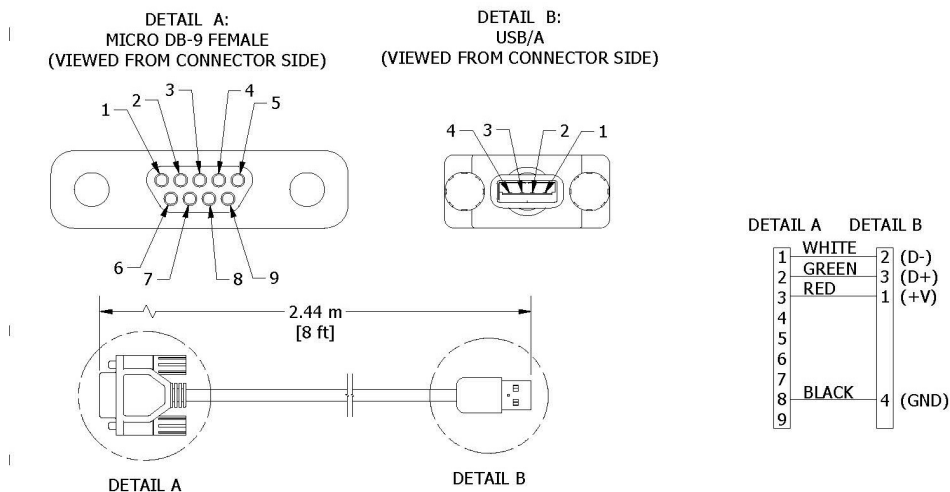
Figure 43 - Communications cable (USB Kits, PN: 9022-0019)
