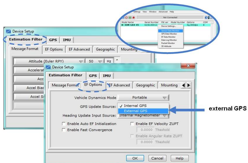
Figure 37 - GPS Source Select
