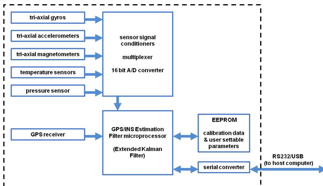
Figure 15 - 3DM-GX4-45™ Block Diagram
