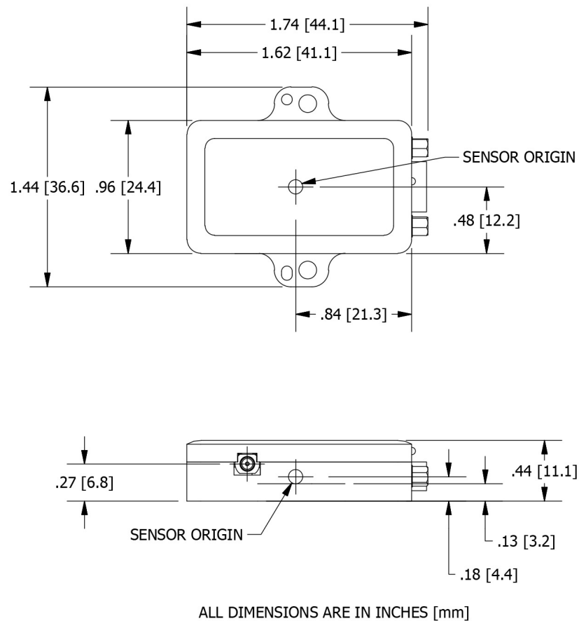
Figure 41 - Sensor Dimensions
