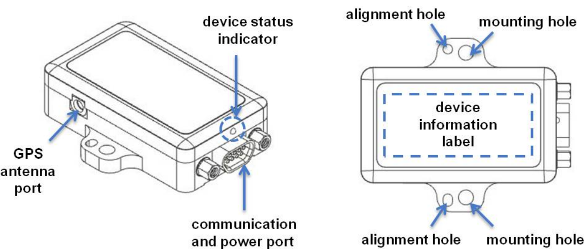
Figure 2 - Interface and Indicators
