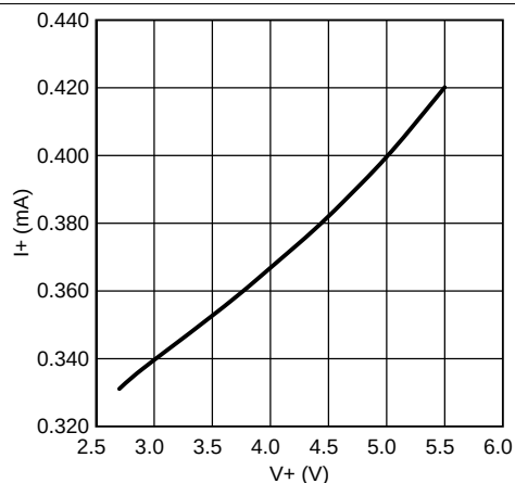
Figure 22. I+ vs. V+ in Shutdown Mode
