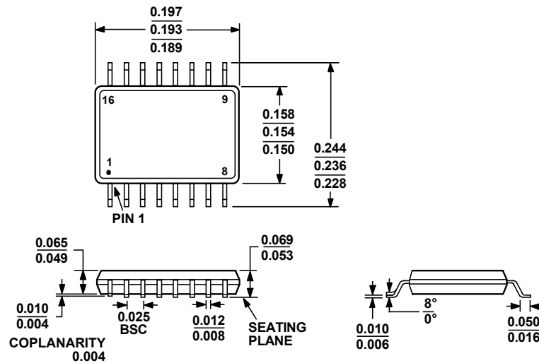
COMPLIANT TO JEDEC STANDARDS MO-137-AB Figure 16. 16-Lead Shrink Small Outline Package [QSOP] (RQ-16) Dimensions shown in inches
