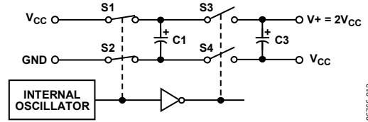
Figure 13. Charge Pump Voltage Doubler
