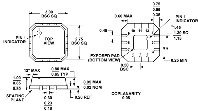
*COMPLIANT TO JEDEC STANDARDS MO-220-VEED-1 EXCEPT FOR EXPOSED PAD DIMENSION. Figure 15. 12-Lead Lead Frame Chip Scale Package [LFCSP_VQ] 3 mm × 3 mm Body, Very Thin Quad (CP-12-1) Dimensions shown in millimeters
