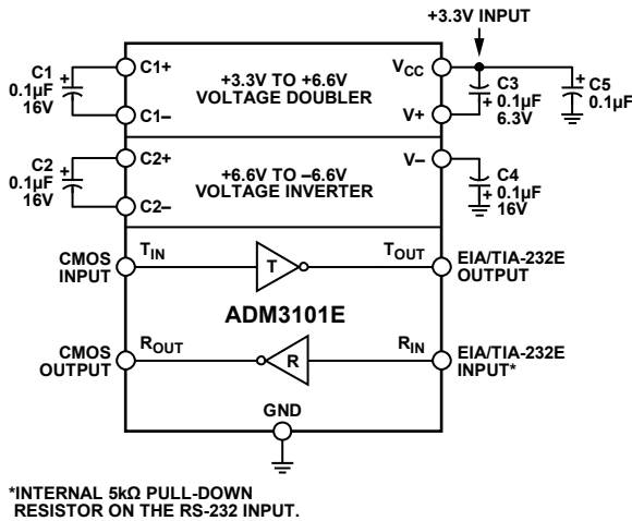
Figure 12. ADM3101E Typical Operating Circuit
