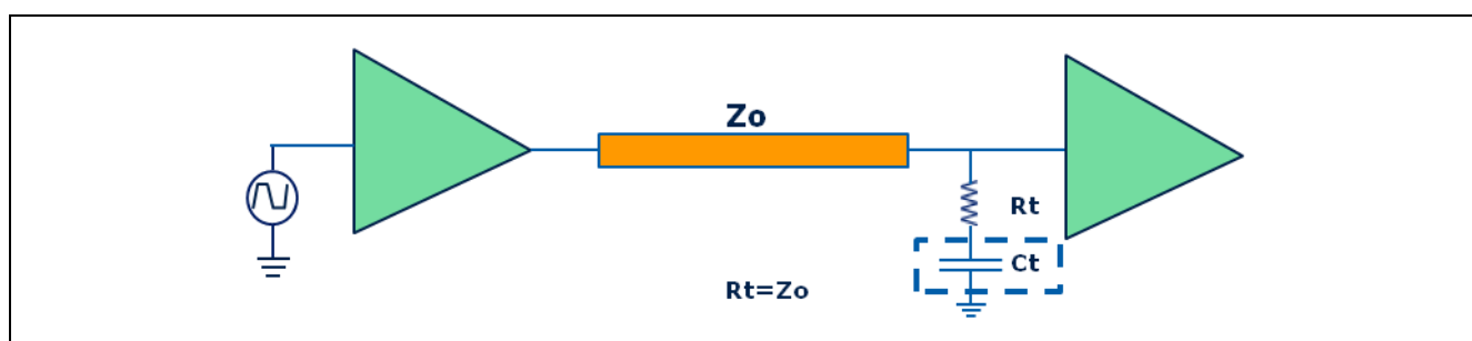
Figure 10 Parallel and AC Termination for Single Ended Lines
