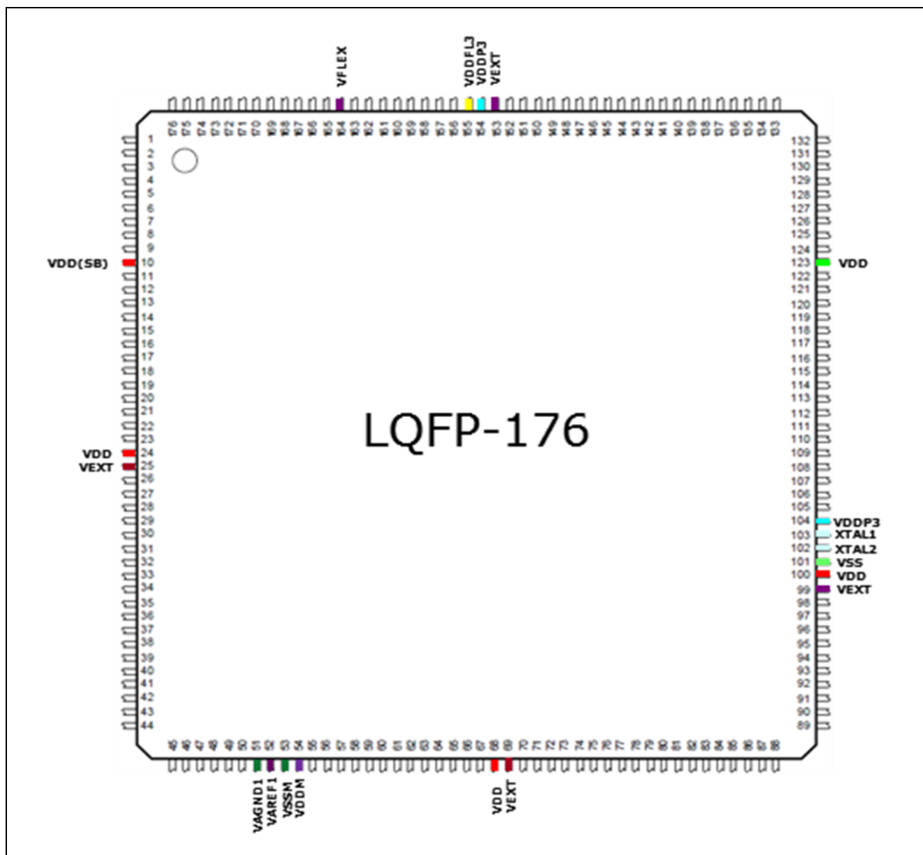
Figure 18 LQFP-176 Package
