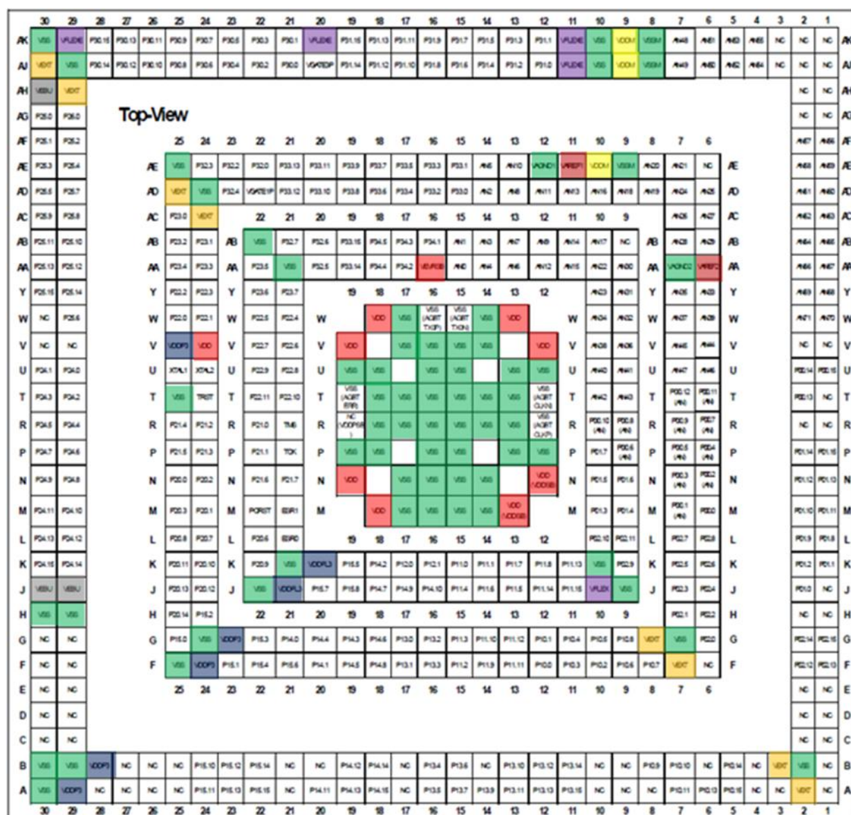
Figure 21 BGA-516
