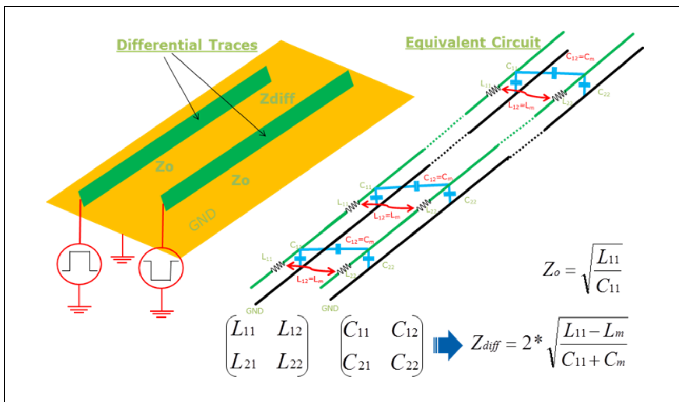
Figure 4 Calculation of the Impedance by using transmission line parameter
