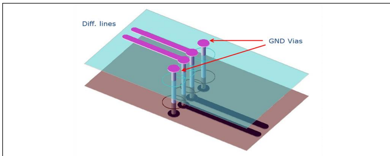
Figure 8 Differential Via
