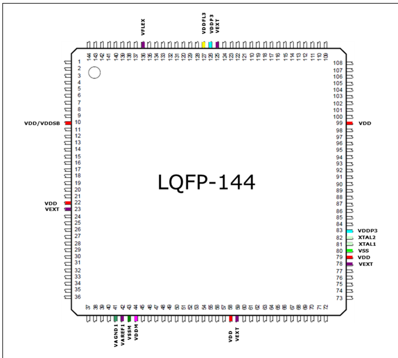
Figure 17 LQFP-144 Package
