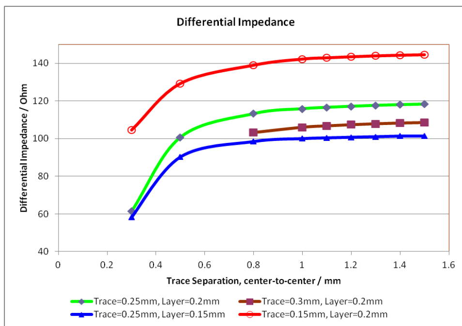
Figure 7 Differential Impedance change with Trace separation
