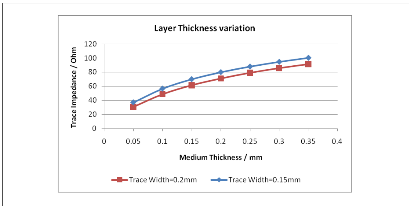
Figure 5 Trace Impedance change with Layer Thickness
