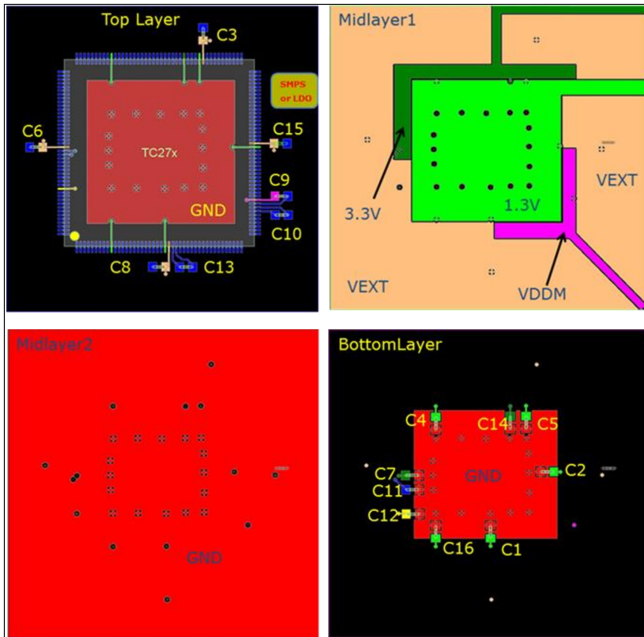
Figure 23 Example Layout for LQFP-176 Package
