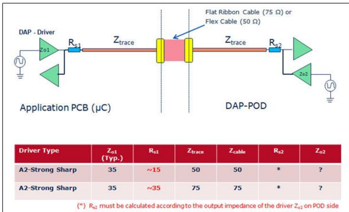
Figure 28 Series Termination of DAP1 and DAP2 (recommendation for 160MHz)
