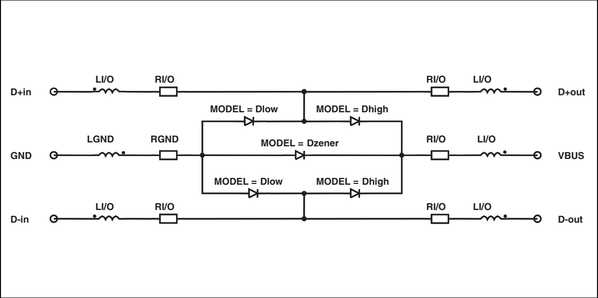
Figure 16. PSpice model
