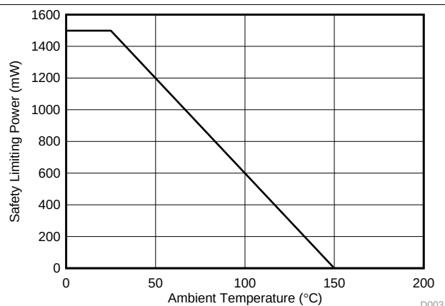
Figure 3. Thermal Derating Curve for Safety Limiting Power for DW-16 Package
