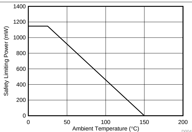
Figure 4. Thermal Derating Curve for Safety Limiting Power for DBQ-16 Package
