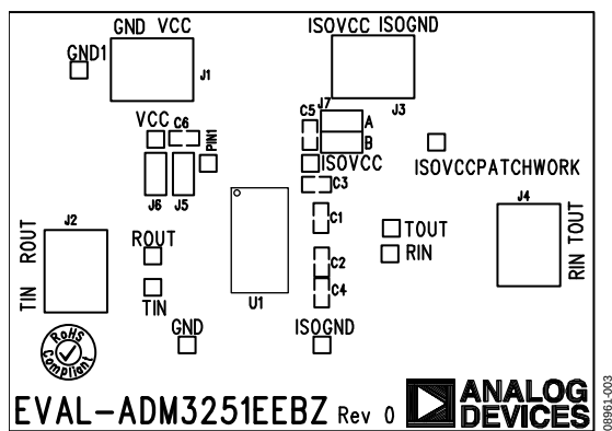
Figure 3. EVAL-ADM3251EEBZ Silkscreen
