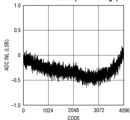
ADC INL vs Code (ADIN Voltage)
