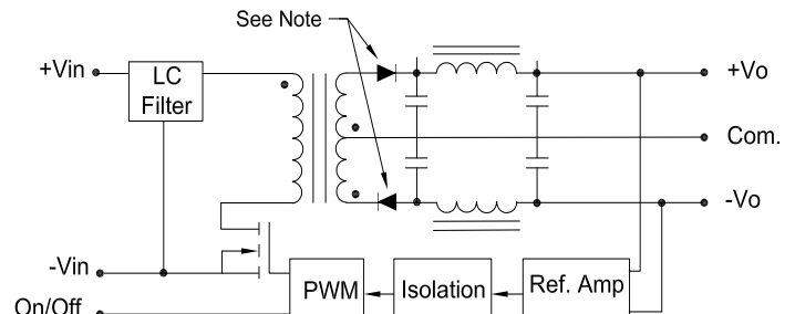
Dual Output Block Diagram
