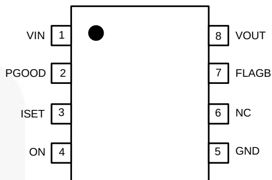
Figure 7. SO8 (Top View)
