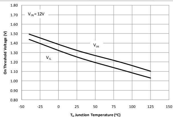
Figure 14. ON Threshold vs. Temperature
