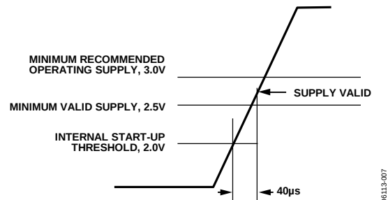
Figure 7. Start-Up Condition, Supply Slew Rate > 12.5 V/ms
