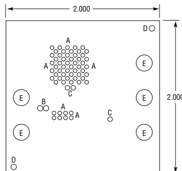
Solder Side
