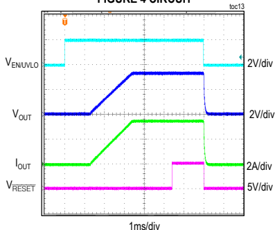
SOFT-START/SHUTDOWN FROM EN/UVLO, 3.3V OUTPUT, 3.5A LOAD CURRENT, FIGURE 4 CIRCUIT toc13
