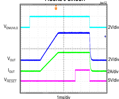
SOFT-START/SHUTDOWN FROM EN/UVLO, 5V OUTPUT, 3.5A LOAD CURRENT, FIGURE 3 CIRCUIT toc12
