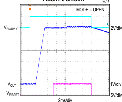
SOFT-START/SHUTDOWN FROM EN/UVLO, 5V OUTPUT, PFM MODE, 5mA LOAD CURRENT, FIGURE 3 CIRCUIT toc14
