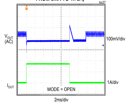
3.3V OUTPUT, PFM MODE, FIGURE 4 CIRCUIT (LOAD CURRENT STEPPED FROM 5mA TO 1.75A)
