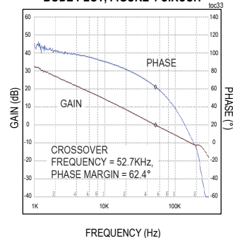
3.3V OUTPUT, 3.5A LOAD CURRENT, BODE PLOT, FIGURE 4 CIRCUIT
