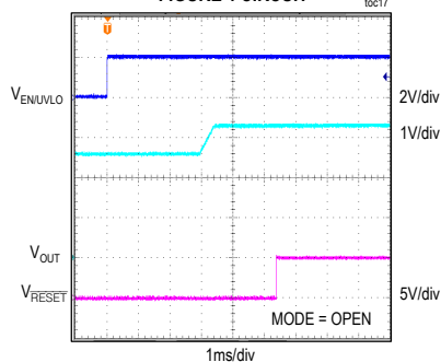
SOFT-START WITH 2.5V PREBIAS, 3.3V OUTPUT, PFM MODE, FIGURE 4 CIRCUIT
