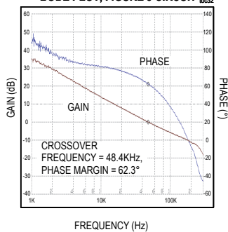
5V OUTPUT, 3.5A LOAD CURRENT BODE PLOT, FIGURE 3 CIRCUIT
