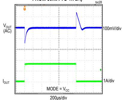
5V OUTPUT, DCM MODE, FIGURE 3 CIRCUIT (LOAD CURRENT STEPPED FROM 50mA TO 1.75A)
