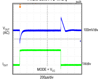
3.3V OUTPUT, DCM MODE, FIGURE 4 CIRCUIT (LOAD CURRENT STEPPED FROM 50mA TO 1.75A)
