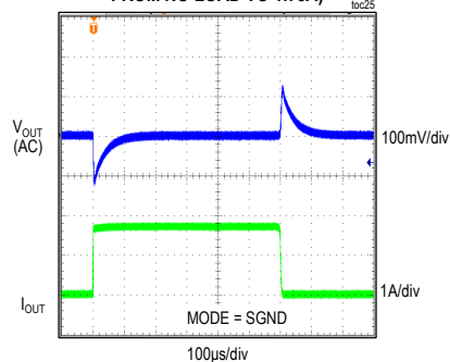
3.3V OUTPUT, PWM MODE, FIGURE 4 CIRCUIT (LOAD CURRENT STEPPED FROM NO LOAD TO 1.75A)
