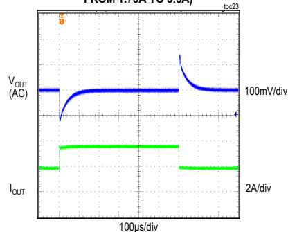
3.3V OUTPUT, PWM MODE, FIGURE 4 CIRCUIT (LOAD CURRENT STEPPED FROM 1.75A TO 3.5A)
