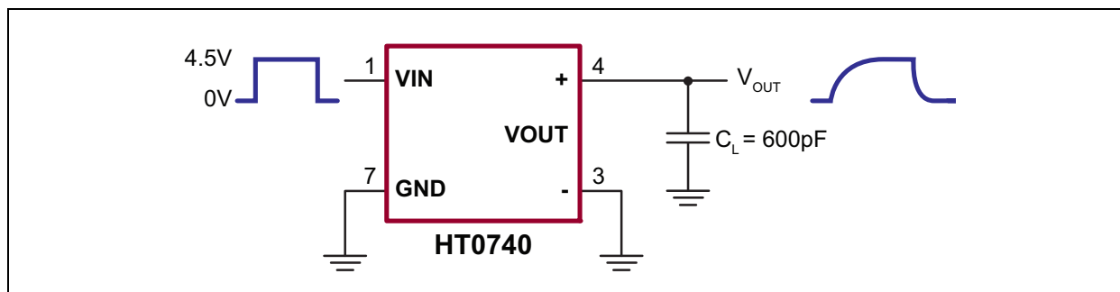
FIGURE 3-2: Test Circuit.
