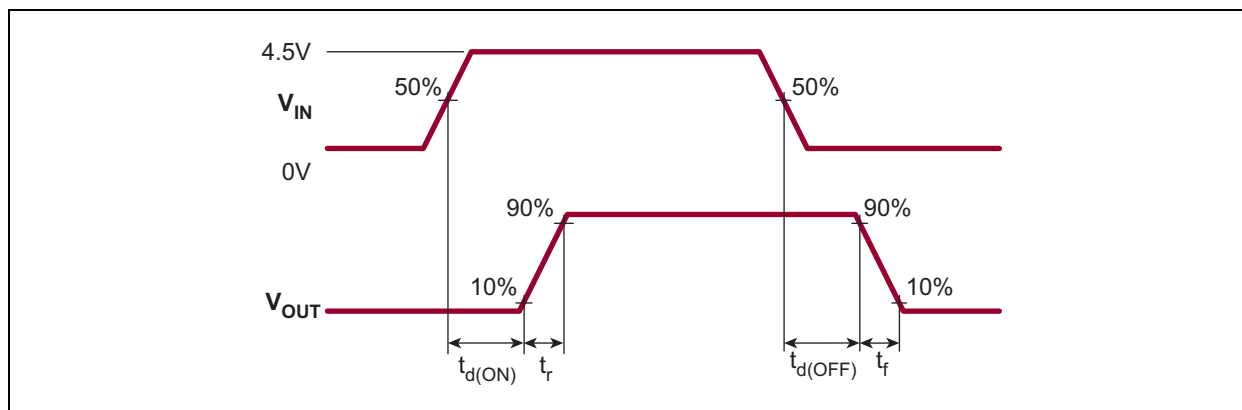
FIGURE 3-1: Timing Waveforms.
