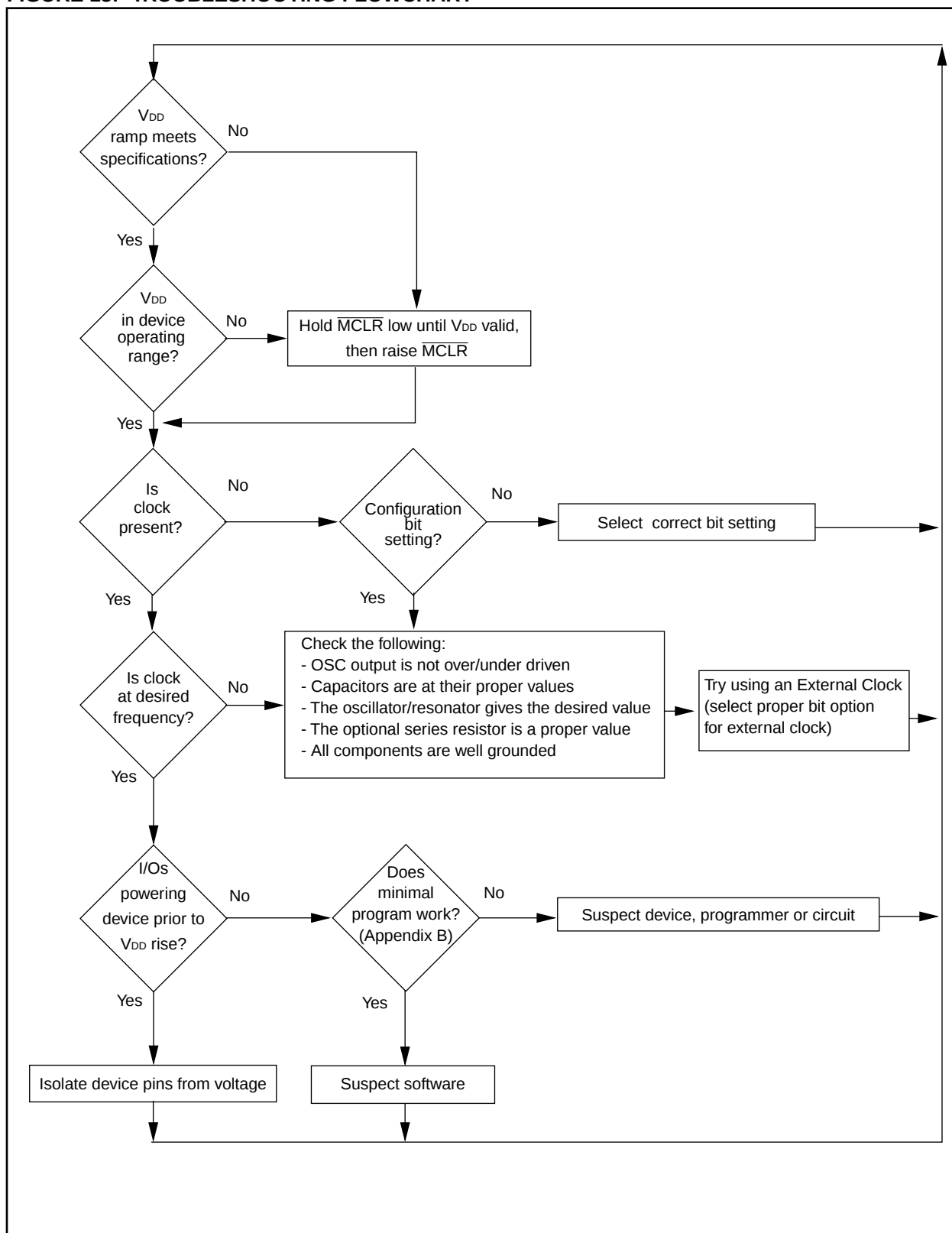
FIGURE 18: TROUBLESHOOTING FLOWCHART
