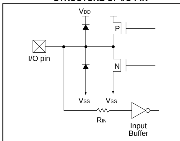
FIGURE 15: TYPICAL ELECTRICAL STRUCTURE OF I/O PIN
