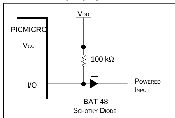
FIGURE 17: POWERED INPUT PROTECTION
