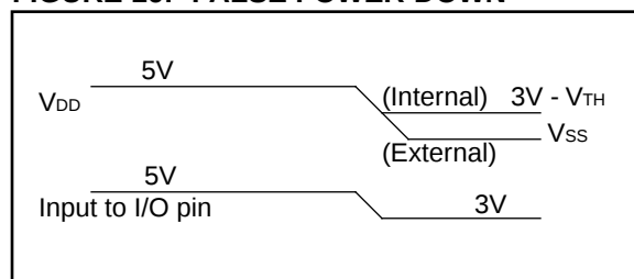
FIGURE 16: FALSE POWER-DOWN
