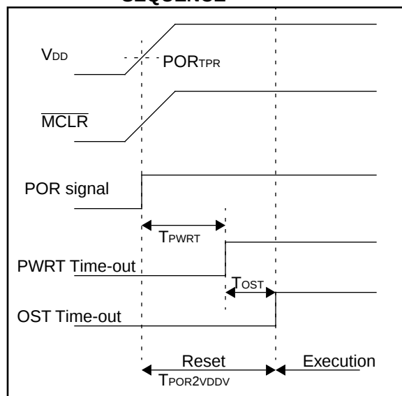
FIGURE 4: START OF DEVICE OPERATION ( MCLR < T_{POR2VDDV} )
