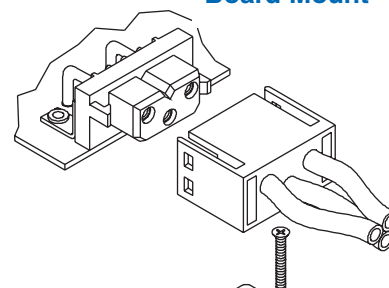
System 5 Cable to Right Angle (90°) Board Mount
