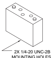
Support Tool
