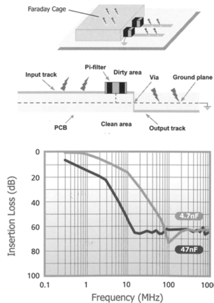
Figure 2. Improved shielding
