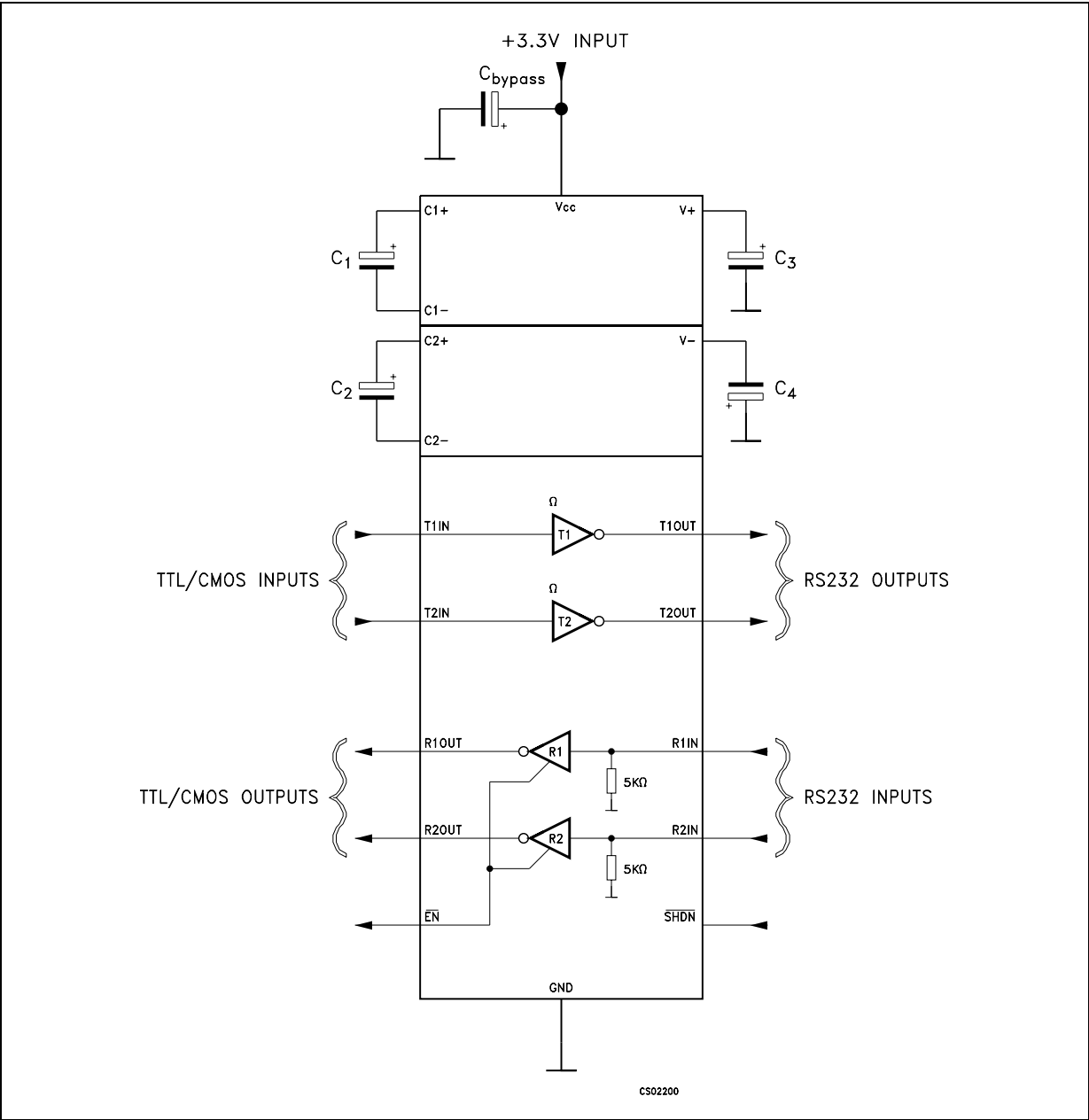
Figure 2. Application circuits
