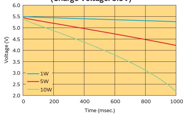
Constant Power Discharge (@25°C) (Charge Voltage: 5.5V)
