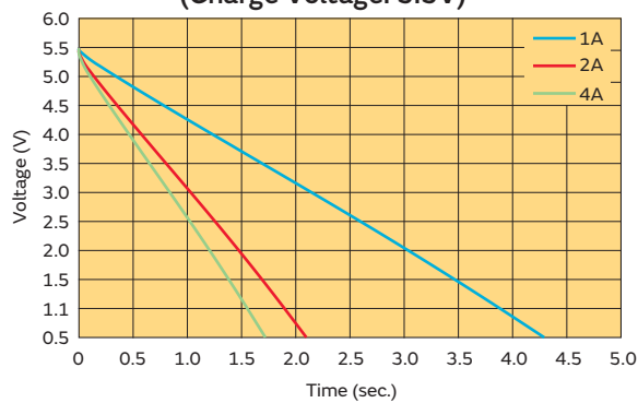
Constant Current Discharge (@25°C) (Charge Voltage: 5.5V)
