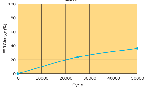
ESR
