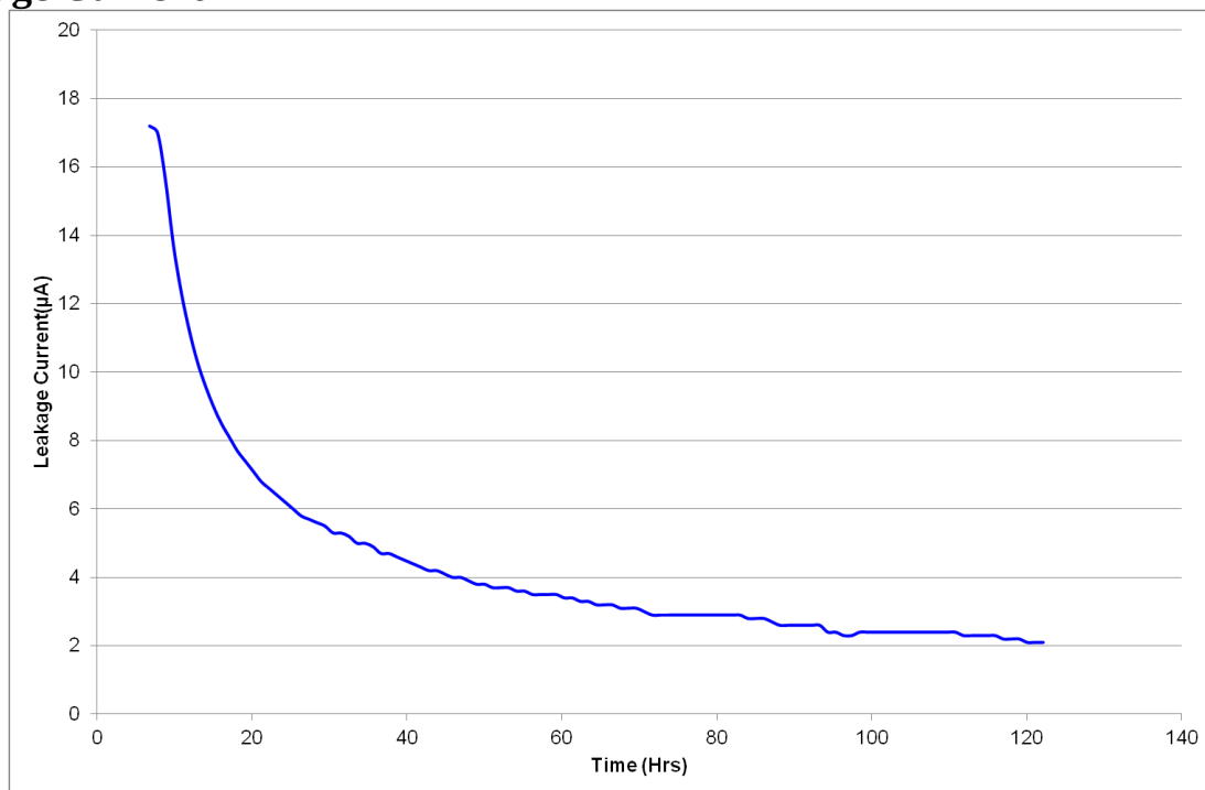
Fig 10: Leakage Current
