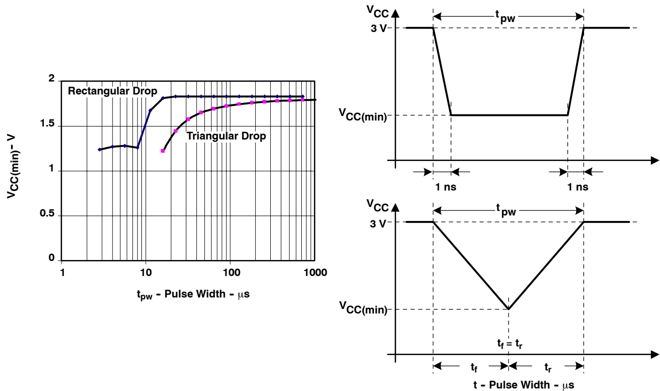
Figure 13. V_{CC(min)} : Square Voltage Drop and Triangle Voltage Drop to Generate an SVD Signal ( VLD = 1 )
