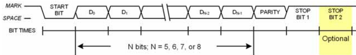
Figure 24.3. UART1 Timing With Parity
