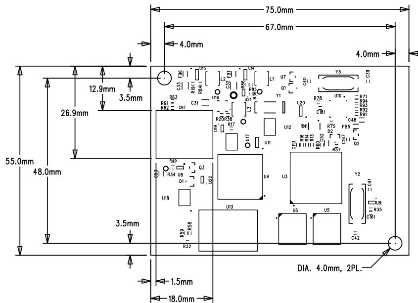
Connector Placement Top View
