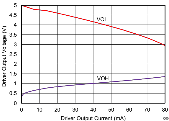
Figure 1. Driver Output Voltage vs Driver Output Current
