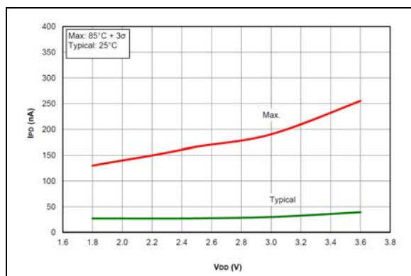
FIGURE 36-13: I_{PD} BASE, Low-Power Sleep Mode, PIC16LF18325/18345 Only
