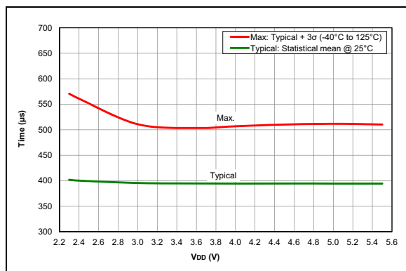
FIGURE 36-113: Wake From Sleep, VREGPM = 1, LFINTOSC, PIC16F18325/18345 Only
