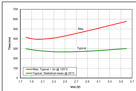
FIGURE 36-88: Comparator Response Time Rising edge, PIC16LF18325/18345 Only
