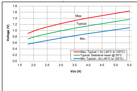
FIGURE 36-99: TTL Trip Thresholds, All devices
