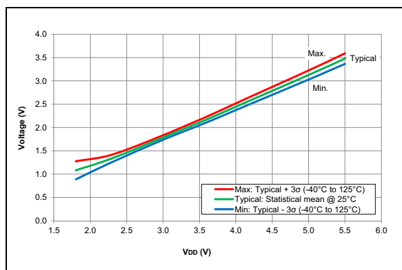
FIGURE 36-97: Schmitt Trigger High Values, All devices
