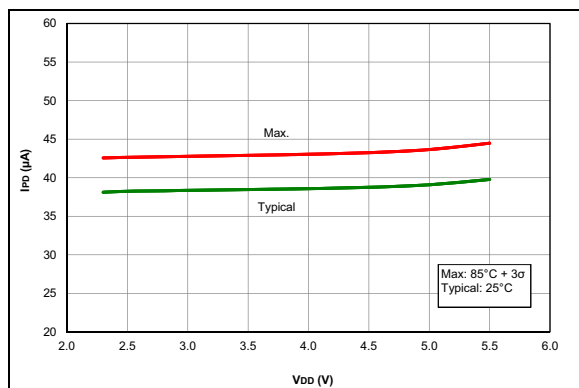
FIGURE 36-17: I_{PD} , Fixed Voltage Reference (FVR), PIC16F18325/18345 Only
