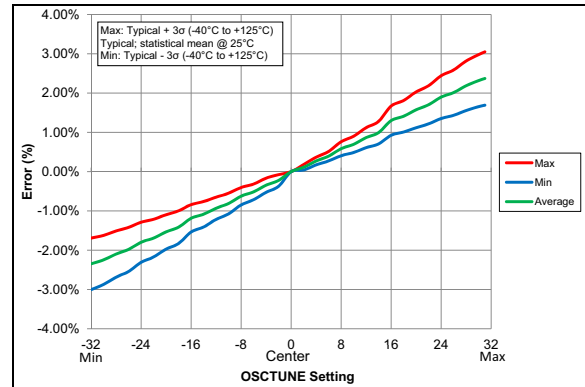
FIGURE 36-104: OSCUNE Center Frequency, PIC16LF18325/18345 Only
