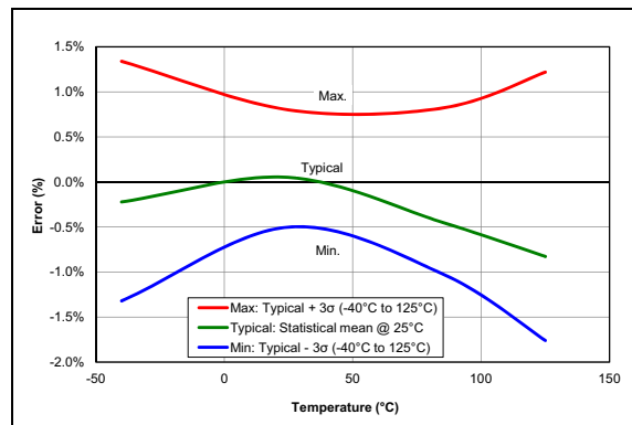
FIGURE 36-28: HFINTOSC Frequency Error V DD = 3V, All devices
