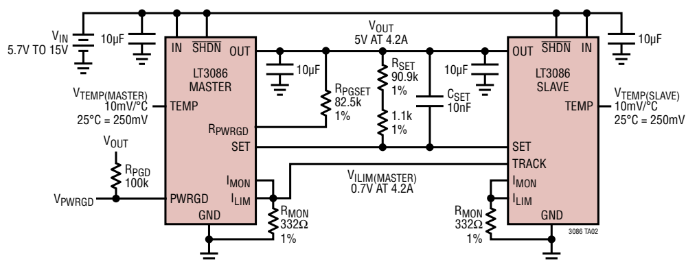
Paralleling Two Regulators for 5V, 4.2A
