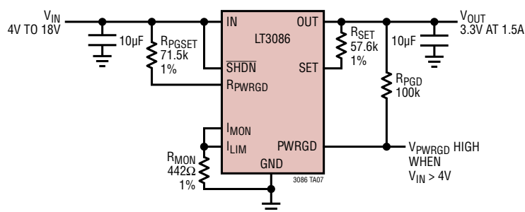
Programming Thermal Limit Temperature
