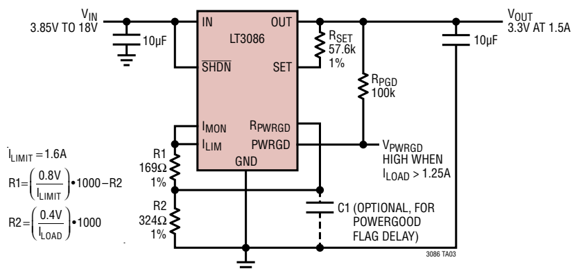
Input Undervoltage Detector Using Power Good
