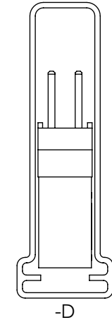
FIG 6 ESQ-110-XX-X-D IN PROCESS "A" (LEAD STYLE -12-T, -13, -14, -23, -24, -33, -34, -44, -37-T, -38, -48, -49, -58, -59, -69)
