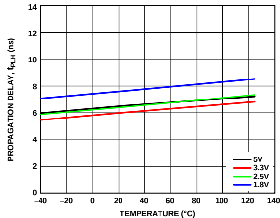
Figure 8. Propagation Delay for Logic High Output ( t_{PLH} ) vs. Temperature at Various Voltages
