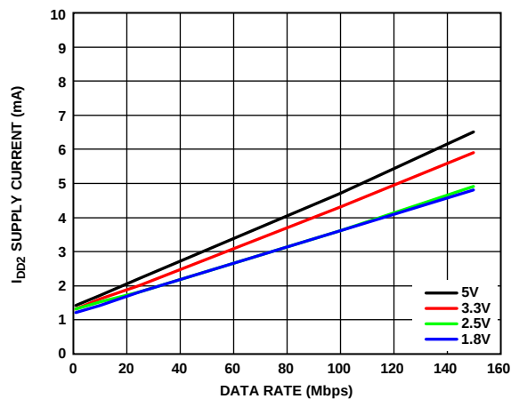
Figure 7. ADuM120N I_{DD2} Supply Current vs. Data Rate at Various Voltages
