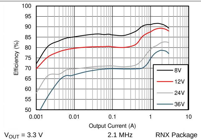
Figure 37. Efficiency
