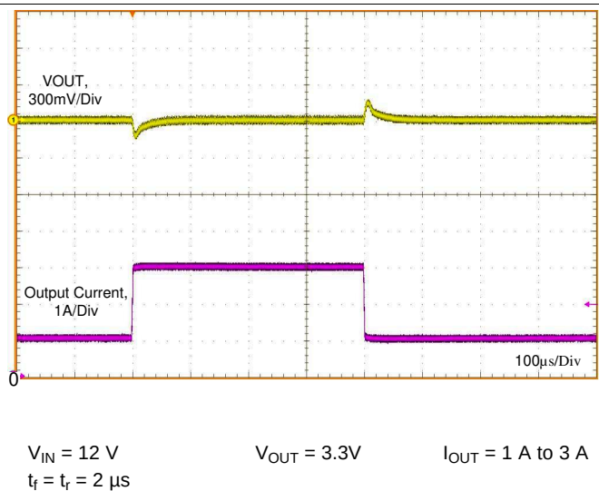
Figure 49. Load Transient
