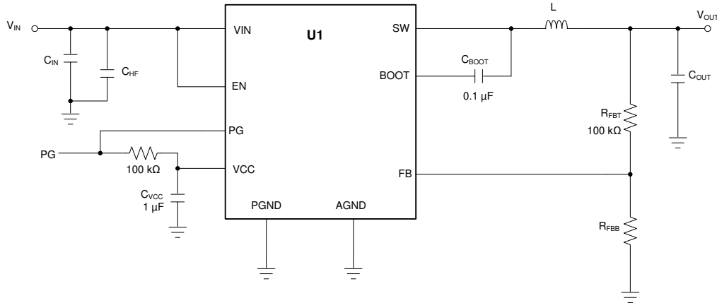
Figure 50. Circuit for Application Curves
