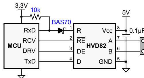
Figure 19. 3V–5V Interface
