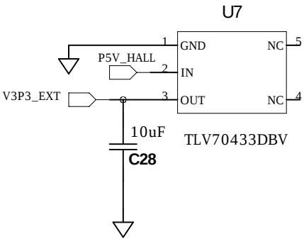
3.3V Power Supply
