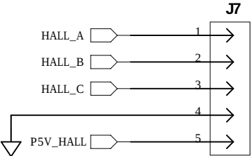
Hall-Effect Sensor Connector
