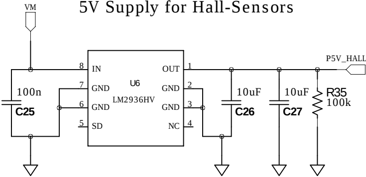
5V Supply for Hall-Sensors
