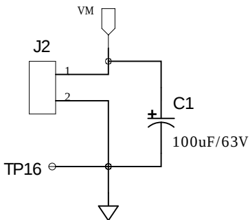
Input Connector
