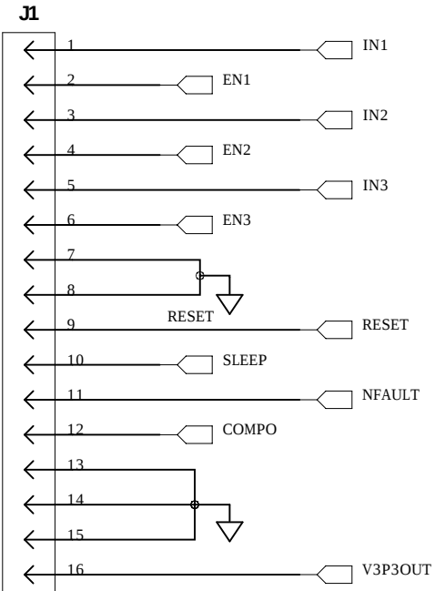
DRV8313 Signal Interface Connector
