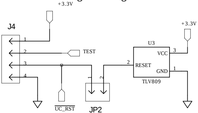
SPI-BY-WIRE Programming Connector
