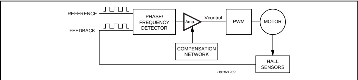
Figure 14. PLL Motor Control.
