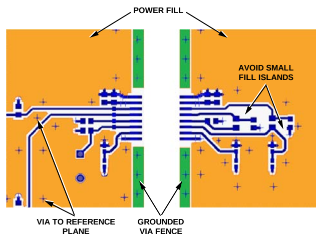
Figure 11. Features of Fill
