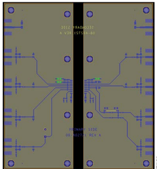
Figure 16. Control Board
