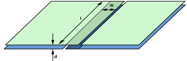
Figure 7. Overlapping Plane Stitching Capacitance
