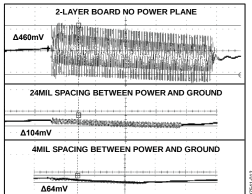
Figure 12. V_{DD} Voltage Noise for Various Stack-Up Options
