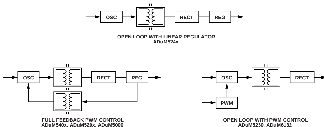
Figure 1. isoPower Architectures
