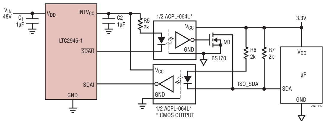
Figure 17. Opto-Isolation of I²C Interface with Low Power, High Speed Opto-couplers (SCL Omitted for Clarity)
