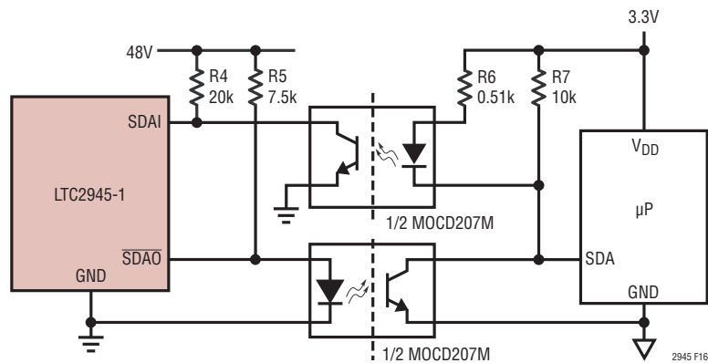
Figure 16. Opto-Isolation of a 1.5kHz I²C Interface Between LTC2945-1 and Microcontroller (SCL Omitted for Clarity)
