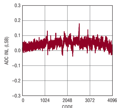
ADC Integral Nonlinearity (ADIN)
