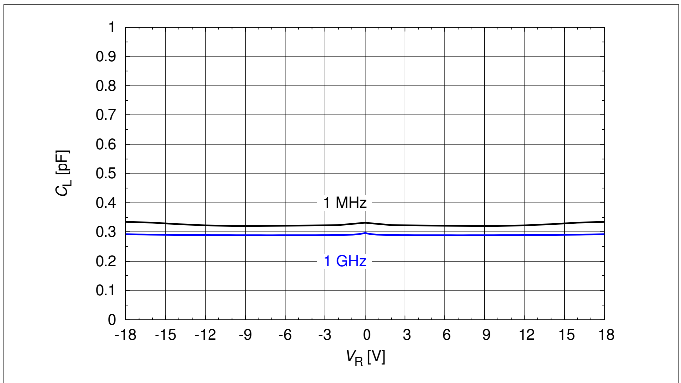
Figure 4 Line capacitance: C_L = f(V_R) , f = 1\text{ MHz}, 1\text{ GHz}
