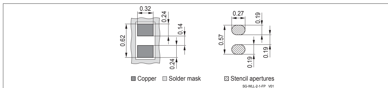
Figure 14 WLL-2-1 footprint
