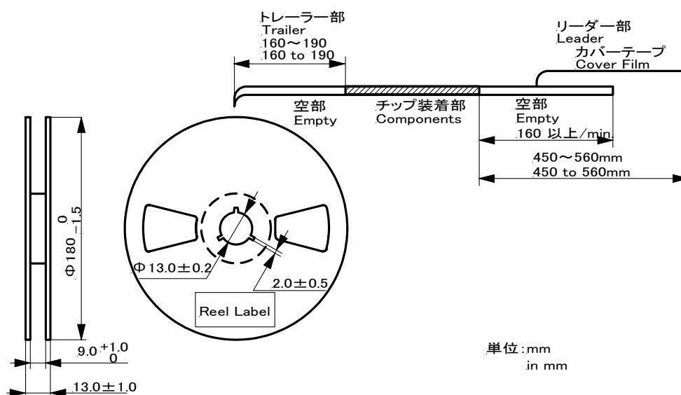
Figure 2. Dimensions of Plastic Tape
