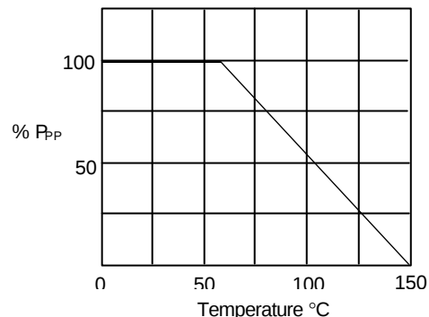
Figure 4 - Derating Curve
