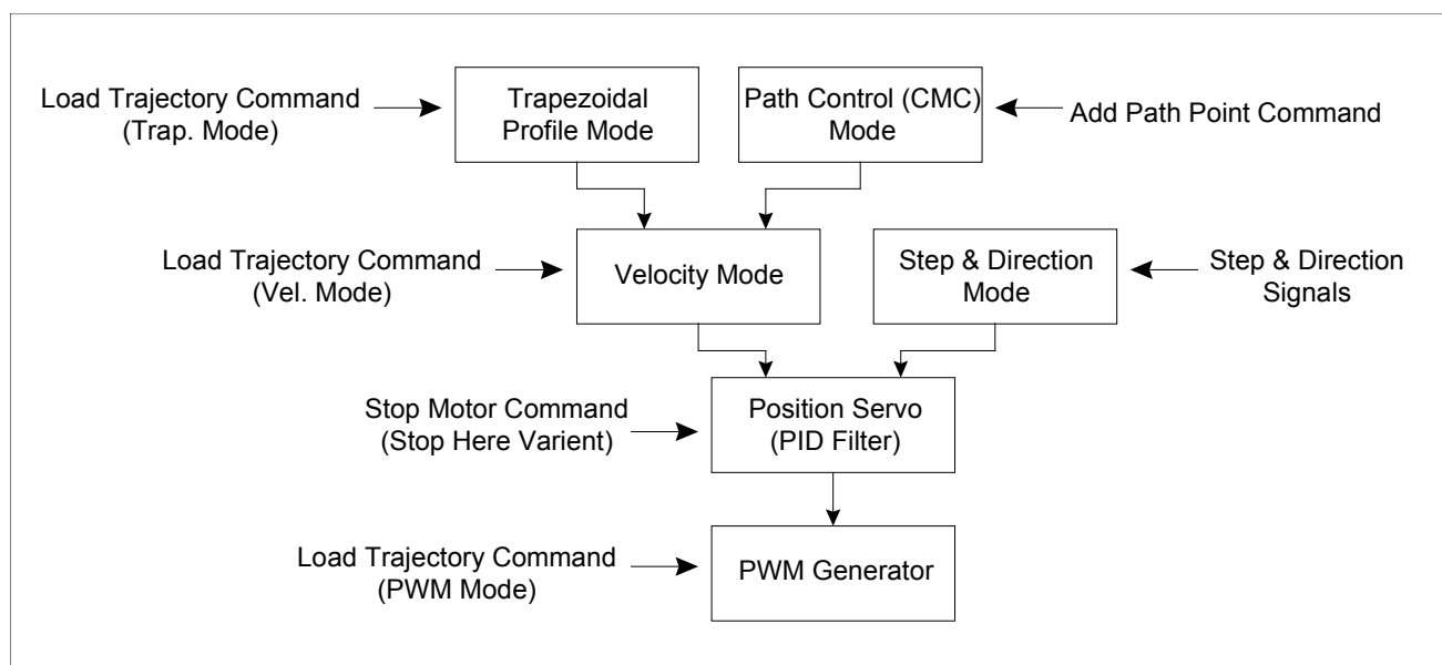
Figure 4 - Levels of control within the PIC-SERVO SC
