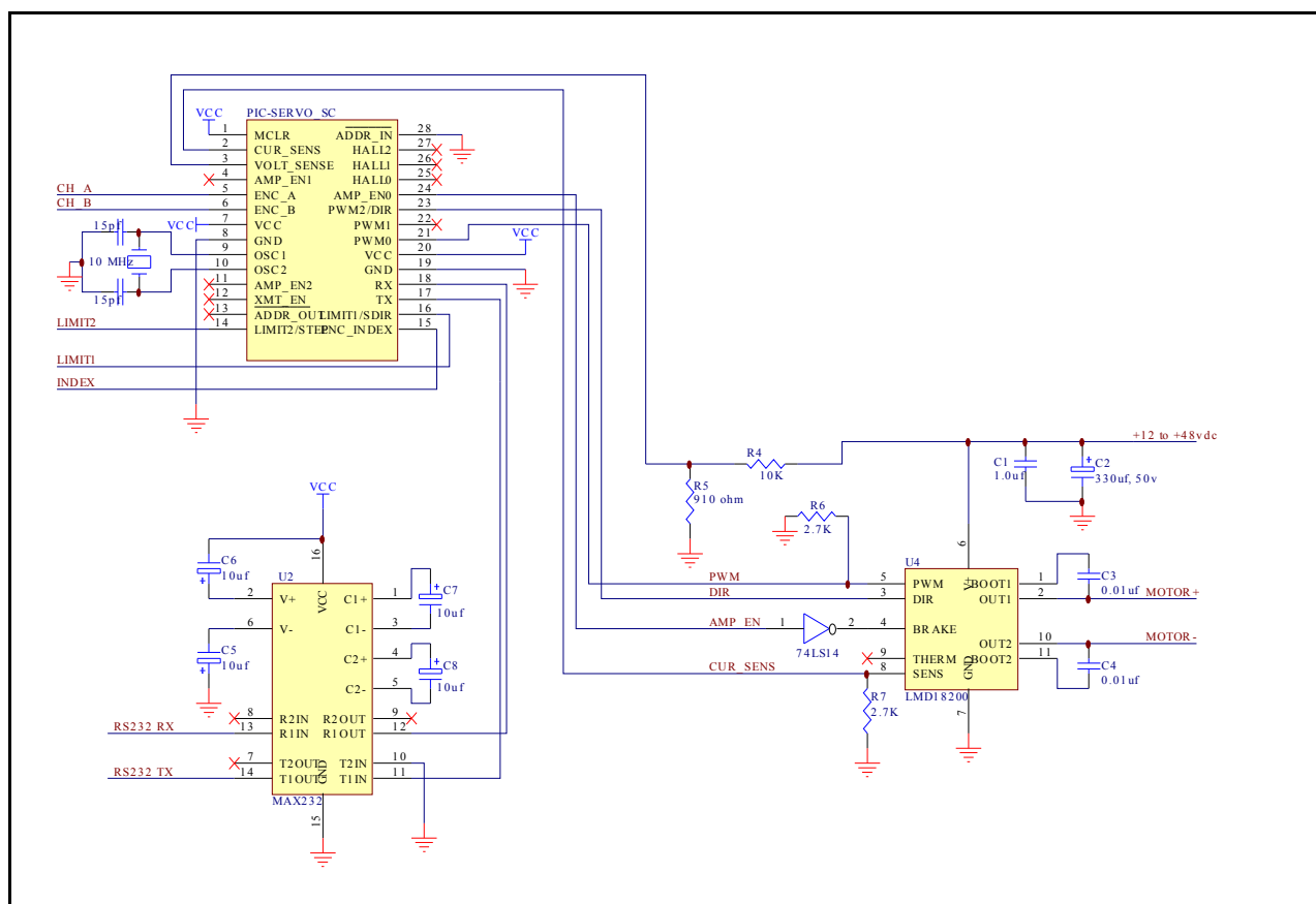
Figure 7 - PIC-SERVO SC controller with RS232 communications
